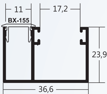
BX-155 2,150 Kg/BARRA 6m
