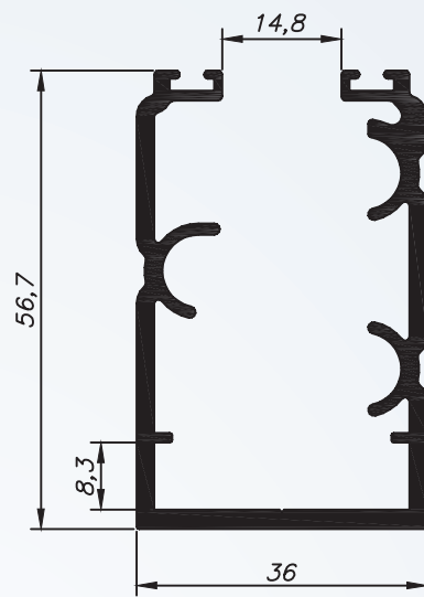
JP-026 6,800 Kg/BARRA 6m
