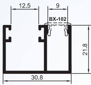
BX-102 1,950 Kg/BARRA 6m
