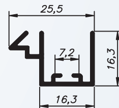
DS-1391 1,310 Kg/BARRA 6m
