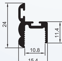
BX-209 1,500 Kg/BARRA 6m
