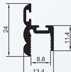
BX-261 1,390 Kg/BARRA 6m
