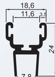
BX-132 1,570 kg/BARRA 6m
